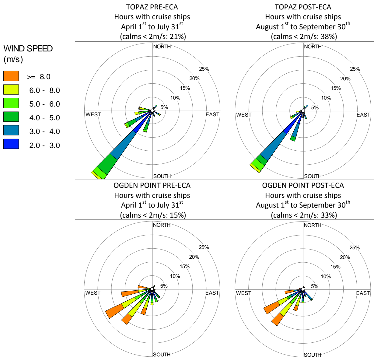
Figure 35. Wind speed and direction pre and post ECA – hours with cruise ships - 2012
