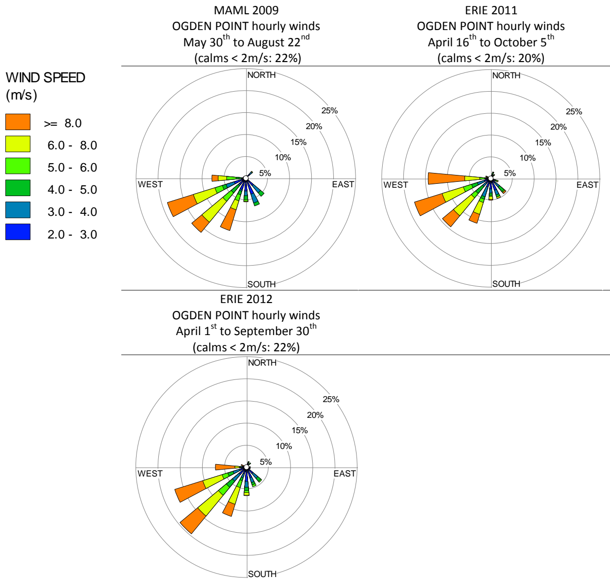
Figure 29. Wind speed and direction at Ogden Point – hours with cruise ships in 2009 - 2012
