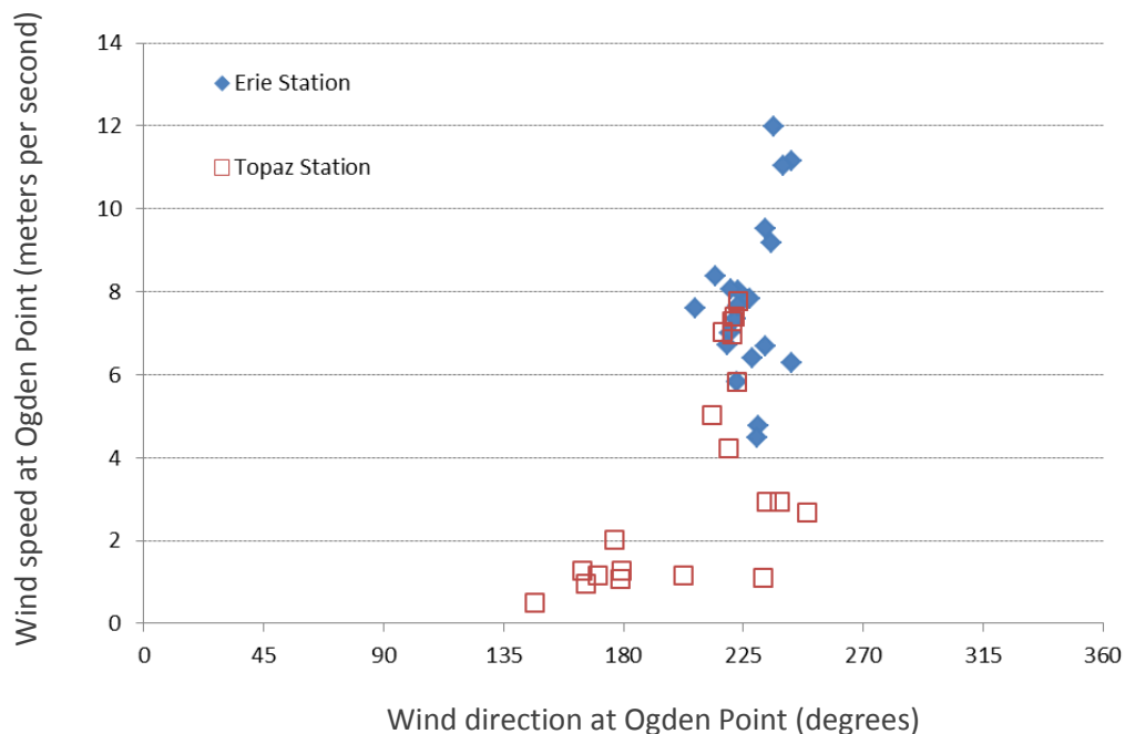
Figure 14. Wind speed and direction at Ogden Point during highest twenty 1 hour averages at Erie and Topaz Stations – 2012
