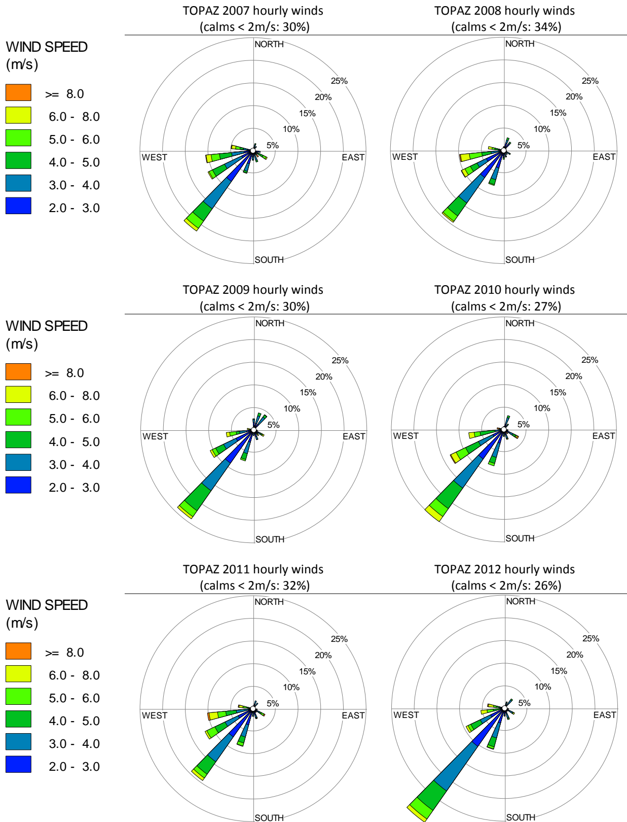
Figure 22. Wind speed and direction for hours with cruise ships - Topaz 2007 to 2012
