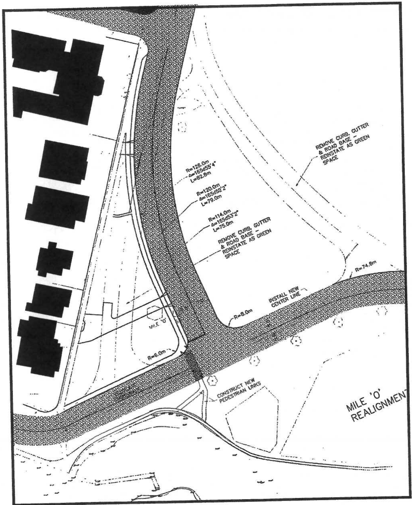
MILE ZERO SITE ROAD ALIGNMENT - option 1
